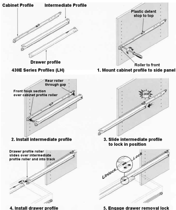
Full extension slides
